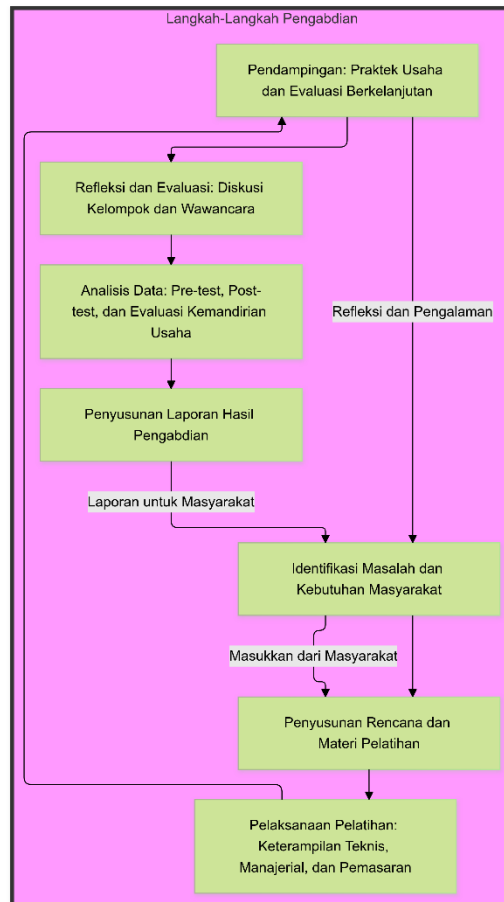
Figure 1 flowchart penngabdian
